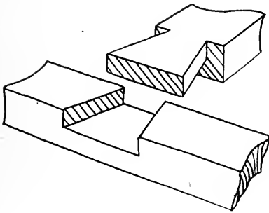
LAPPED DOVE-TAIL
